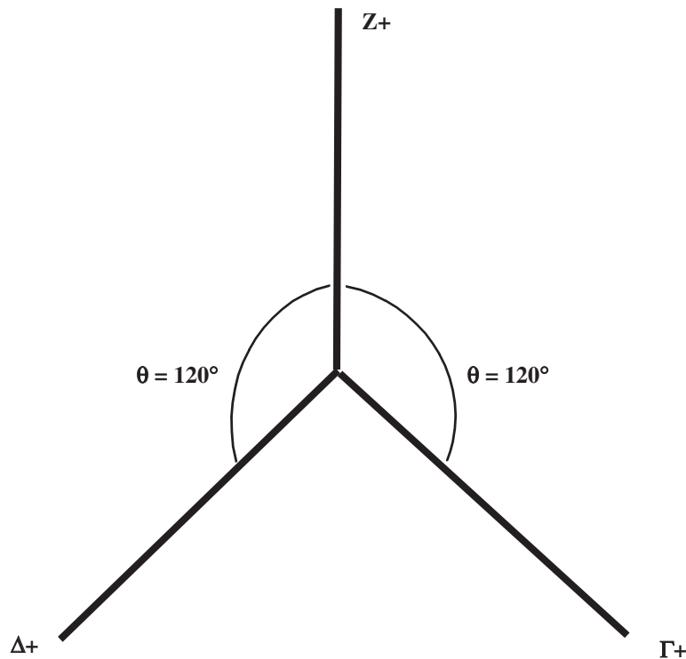
Fig. 4. Stern-Gerlach angles for spin measurements in the Y-Z plane.
