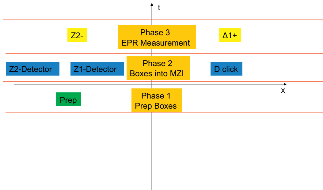
Fig. 6. Experimental sequence consistent with a spin measurement in the Z direction after a D click.
