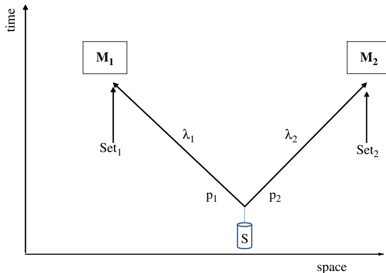
Fig. 3. Schematic spacetime diagram of basic EPR experiment.
