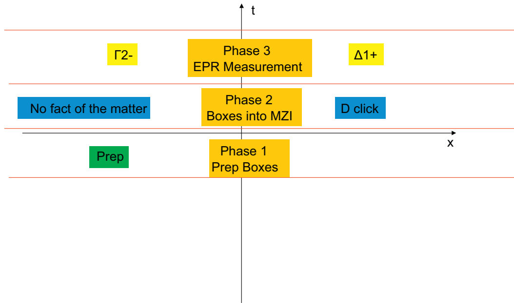
Fig. 5. Experimental sequence consistent with no spin measurements in the Z direction after a D click.
